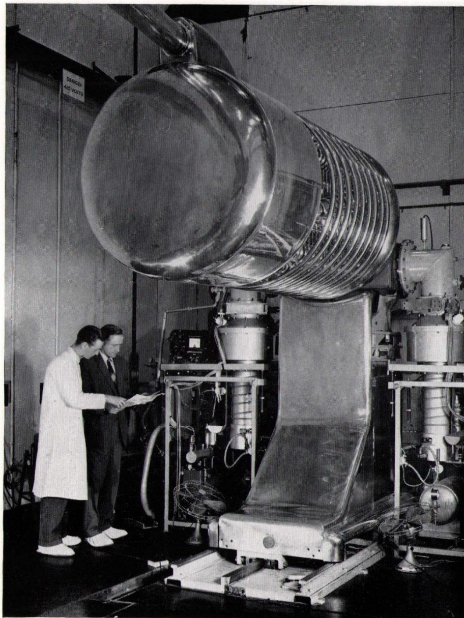
High-voltage ion gun in which protons are focused into a beam prior to entering the injector of Nimrod
