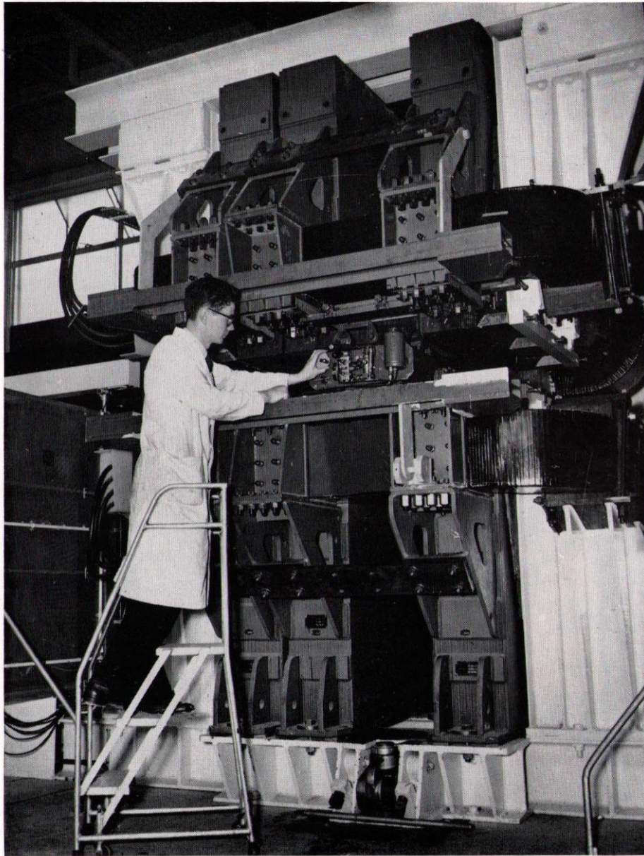
Testing rig for measuring magnetic properties of Nimrod magnet sectors
