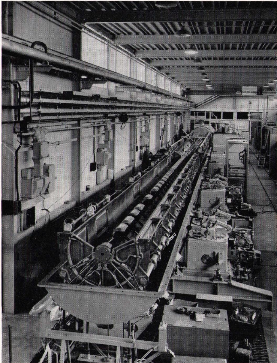
Exposed view of drift tubes in tank III of the 50 MeV Proton Linear Accelerator
