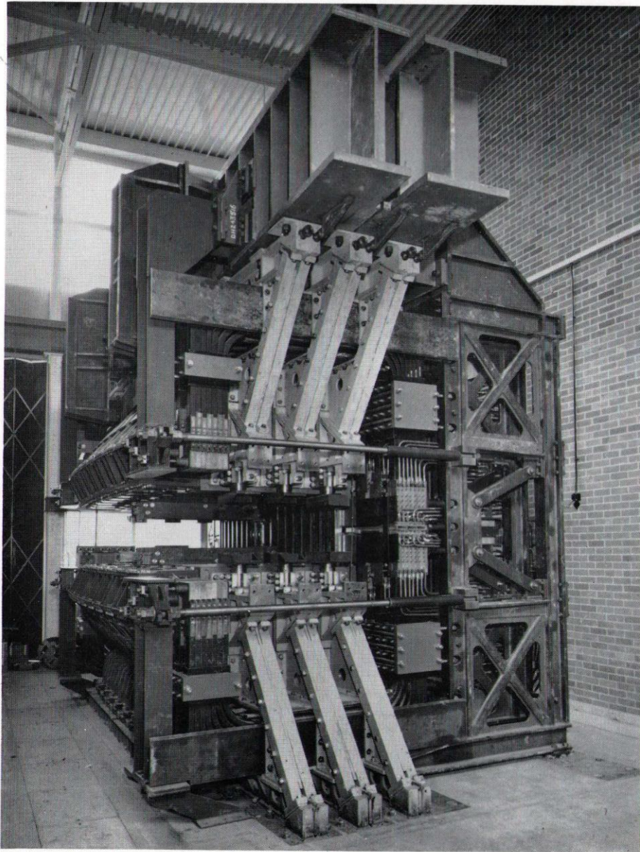
Full scale model of a section of the Nimrod magnet built to test various features of the design.
