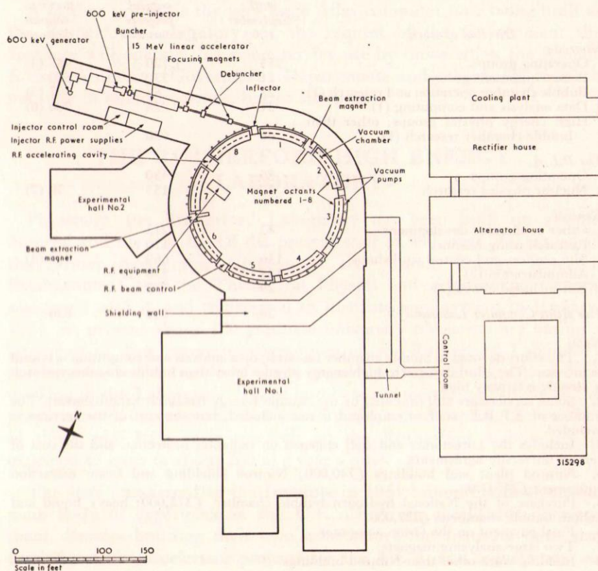
FIG. 1. Plan of Nimrod
