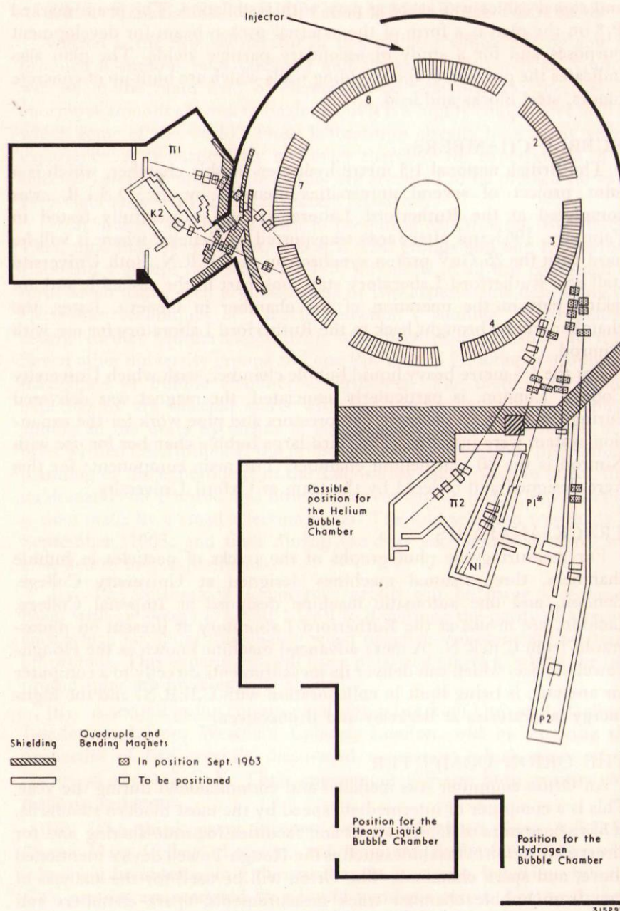
FIG. 2. Plan showing the positions of the first beams in the Nimrod experimental areas.
