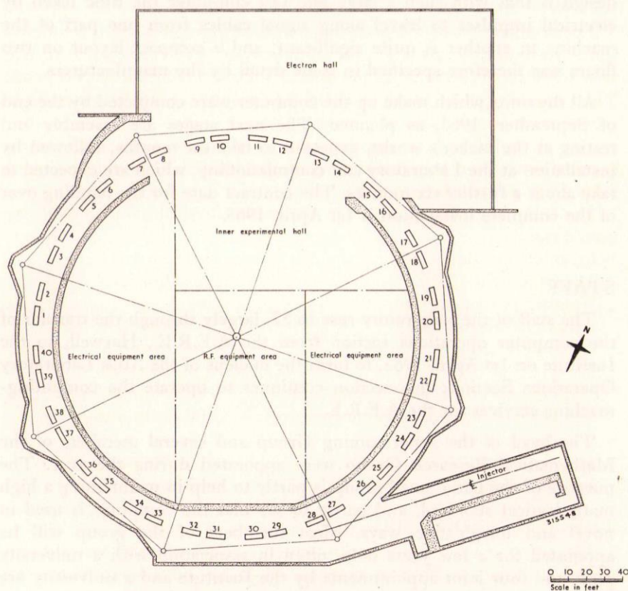
FIG. 4. NINA. Plans showing the general arrangement
