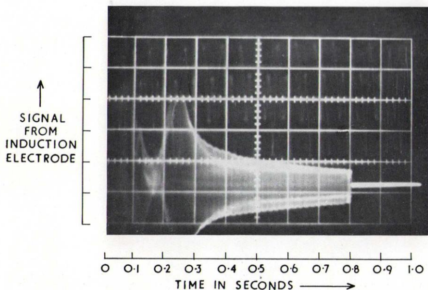
PHOTOGRAPH OF AN OSCILLOSCOPE TRACE MADE ON 27th AUGUST, 1963, SHOWING ACCELERATION OF PROTONS TO 8 GeV IN NIMROD.
