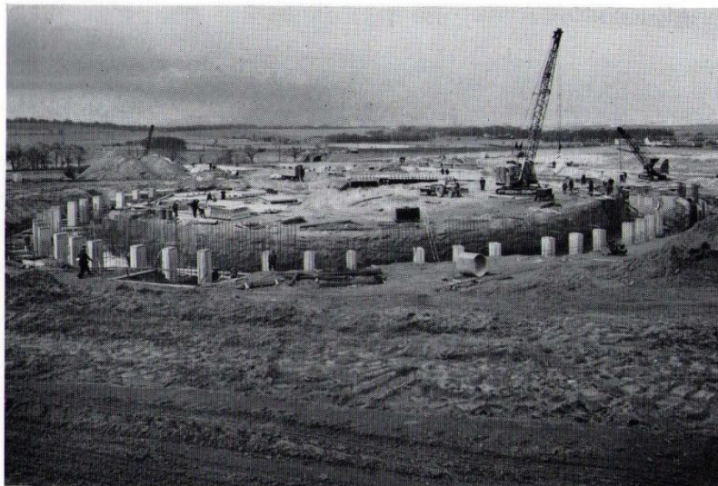
Nina magnet foundations
