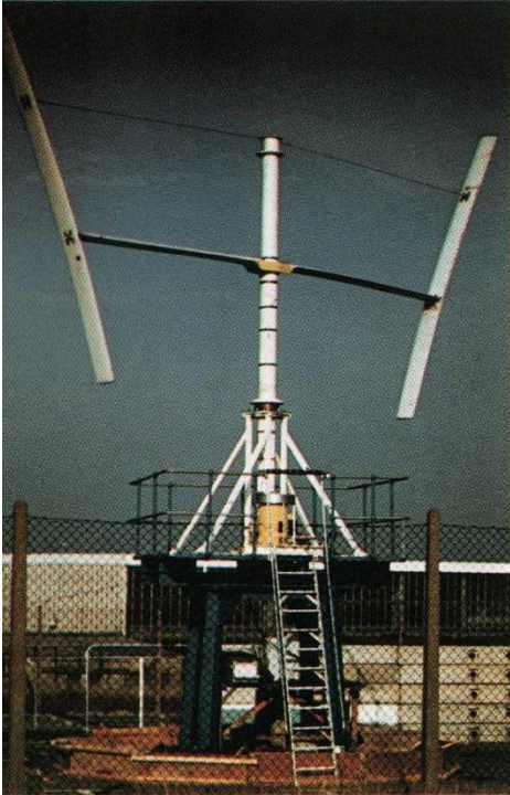
A 6.5 kilowatt aerogenerator built at Chilton for Cambridge University.
