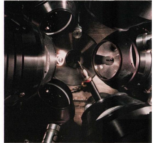
An interior view of the six-beam target chamber, used for laser compression experiments.
