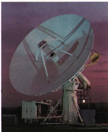
The 12m diameter antenna which is being set up to track the Infra-Red Astronomical Satellite.
