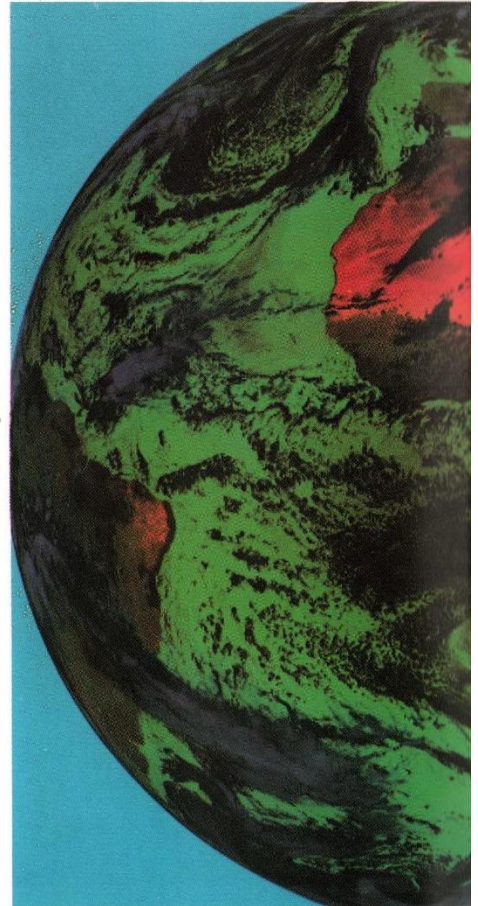
A coloured Meteosat image of the Earth produced by the Interactive Planetary Image Processing System at University College, London. The green shows the "visible" image, red is infra-red radiation and blue is water vapour (Photo: UCL).
