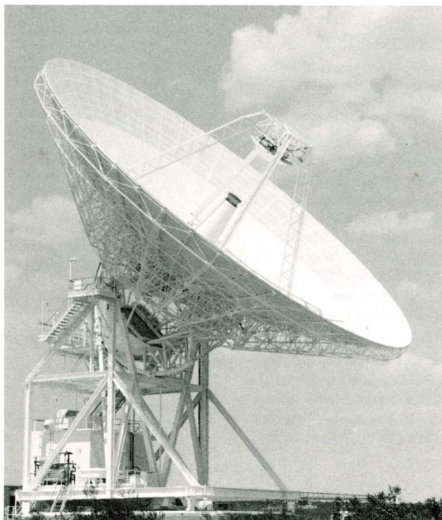
The new-design 34-meter high-efficiency antenna was added to the Goldstone complex in 1984, Canberra in 1985, and Madrid in 1987. The dish surface is "beam-shaped" for maximum signal-gathering efficiency.
