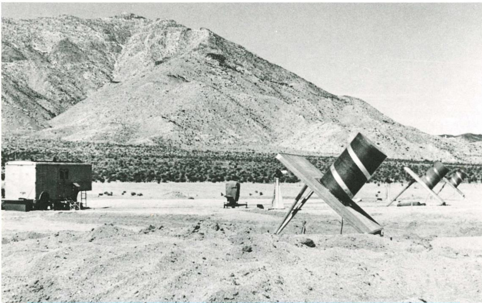
In 1958, JPL's Microlock system, the Deep Space Network precursor, used 5-foot-long helical antennas to track the flight of Explorer 1, the first successful U.S. satellite.
