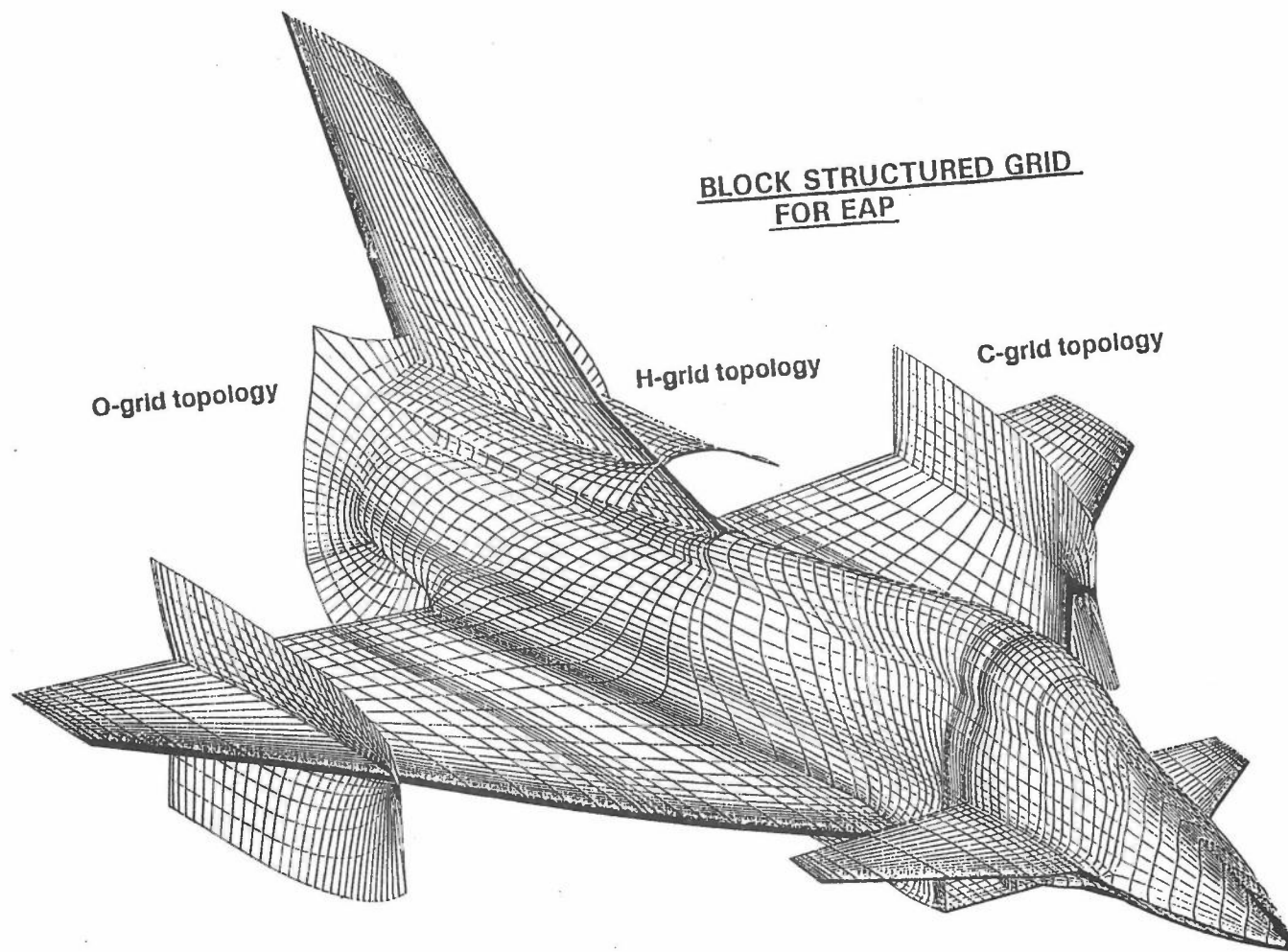
Figure 1: Block Structured Mesh for EAP (Courtesy of ARA Ltd, Bedford)
